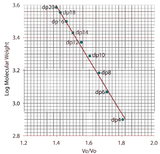
HA Oligosaccharides in Superdex S75; linear correlation of V_e/V_o vs log molecular weight
